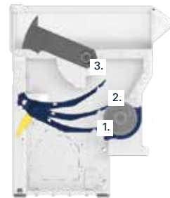
Hydraulic door for maintenance and removal of foreign objects
